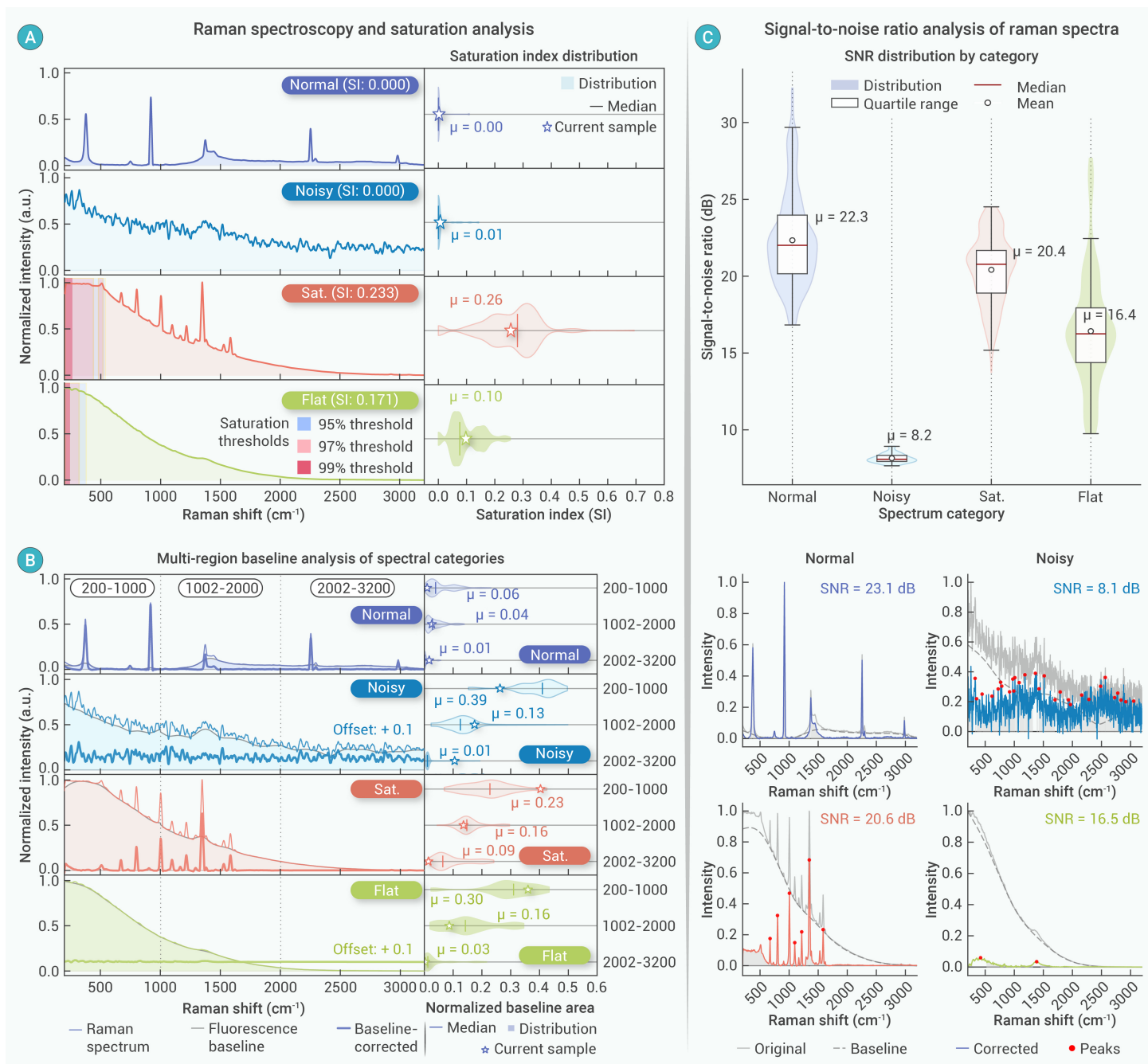
Figure 4. Visualization and statistical analysis of physics-informed quality metrics (A) Saturation Analysis (SI): Comparison of spectral morphologies (Left) shows distinct “flat-top” plateaus in saturated spectra compared to normal peaks. The SI distribution (Right) confirms significantly higher values for the Saturated class. (B) Baseline Analysis (SBI): Multi-region segmentation (200-1000, 1002-2000, 2002-3200 cm -1 ) reveals that Flat spectra possess significantly larger baseline areas due to fluorescence. (C) Noise Analysis (NI): Signal-to-Noise Ratio (SNR) distributions demonstrate that the Noise Index derived from SNR effectively separates Noisy spectra (mean SNR ≈ 8.2 dB) from other categories.
