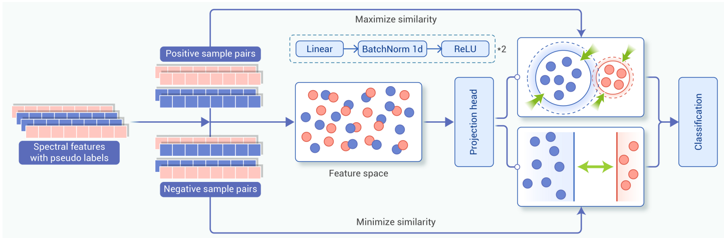
Figure 3. Schematic diagram of the contrastive learning strategy.
