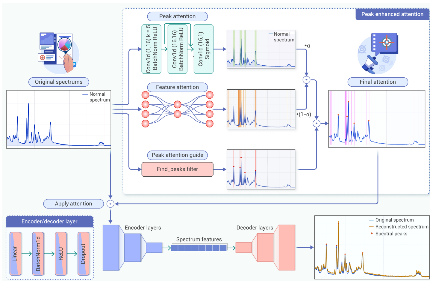
Figure 2. Architecture of the Peak-attention enhanced Autoencoder.
