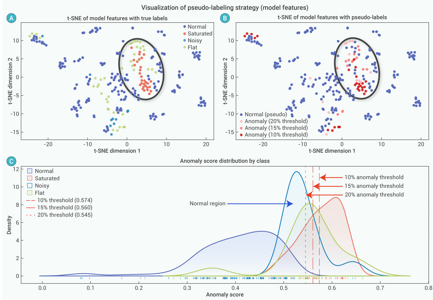
Figure 6. Visualization of pseudo-label generation mechanism (A) t-SNE visualization of model features colored by true labels, highlighting the inherent overlap between classes. (B) t-SNE visualization colored by generated pseudo-labels, illustrating the "easy-to-difficult" curriculum: the 10% threshold identifies the core Saturated cluster, while the 15% and 20% thresholds progressively expand to include boundary Noisy and Flat samples. (C) Anomaly score distributions for each true class. The vertical lines indicate the dynamic thresholds corresponding to the 10%, 15%, and 20% anomaly ratios, demonstrating how the progressive strategy captures samples from high certainty to high ambiguity.
