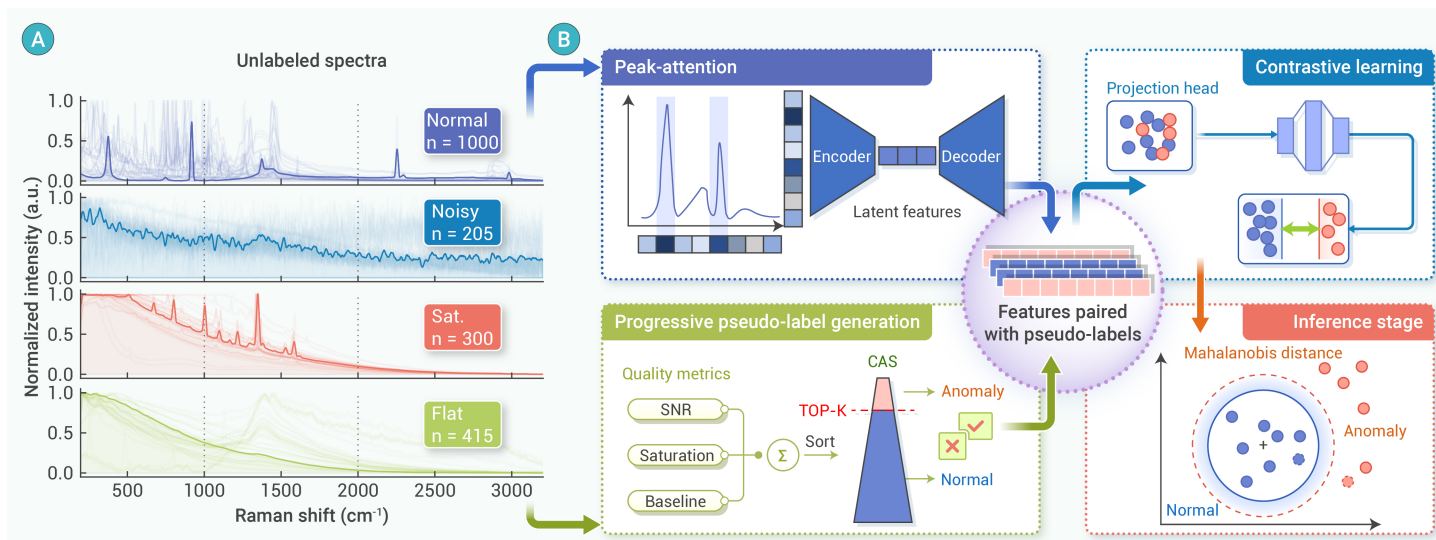
Figure 1. Data Challenges and System Architecture of PAQC framework (A) Representative raw Raman spectra illustrating the four primary categories in the dataset: Normal (high-quality), Noisy (low SNR), Saturated (signal clipping), and Flat (fluorescence interference). (B) The overall workflow of the proposed PAQC hybrid-intelligence framework. It processes unlabeled spectra through two parallel streams: an explicit knowledge stream calculating physics-informed metrics (SI, SBI, NI) to generate high-confidence pseudo-labels, and an implicit knowledge stream utilizing a Peak-Attention Autoencoder to extract deep features. These are fused via a progressive contrastive learning.
