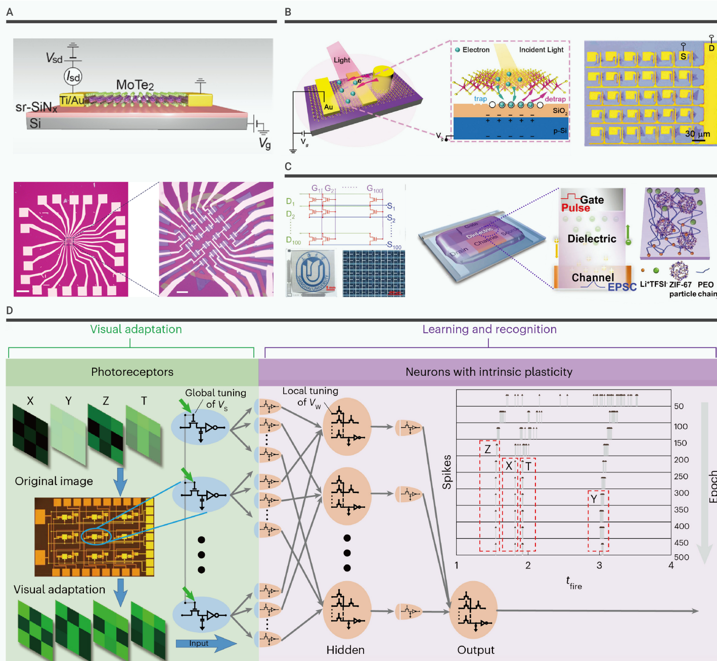
Figure 4. Schematic of the device architecture and working mechanism of a three-terminal artificial synaptic transistor (A) The diagram presents the Sr-SiNx memory configured as a FET, accompanied by an optical image of the constructed synaptic array that includes electrode pads. A scale bar indicates a measurement of 200 \mu\text{m} . Additionally, an enlarged view of isolated synaptic channels is presented with a scale bar measuring 10 \mu\text{m} , featuring a channel length of 4 \mu\text{m} . Reproduced with permission. 33 Copyright 2021, American Chemical Society. (B) This design incorporates a schematic representation of a MoS 2 synaptic transistor integrated with a gold nanorod functioning under light illumination. A substantial number of plasmonic doping electrons can be injected into the MoS 2 monolayers, enhancing the photocurrent efficiency. An enlarged view illustrates how electrons are trapped or released at the MoS 2 /SiO 2 interface, elucidating the operational mechanism of synaptic behaviors. An optical image showing the electrodes arrayed on the MoS 2 monolayers is also included, with a scale bar of 30 \mu\text{m} . Reproduced with permission. 34 Copyright 2023, Wiley - VCH. (C) The illustration features a circuit diagram, a photograph and a micrograph of the array, which is devoid of electrolyte. This setup integrates 100 \times 100 transistors onto a 2.5 \times 2.5 cm 2 glass substrate, with a badge height of 2.5 cm. The diagram depicts the multilayer and lateral architectures of a single unit of the array, along with the multilayer structures associated with the substrate, drain, source pattern, channel, isolation, gate pattern and electrolyte. Furthermore, it elucidates the mechanism of device conductivity modulation and the transportation of Li + ions. Reproduced with permission. 121 Copyright 2023, Wiley - VCH. (D) Complete BioNN architecture of the in-situ image processing and STDP learning simulation. Reproduced with permission. 128 Copyright 2025, Springer Nature.
