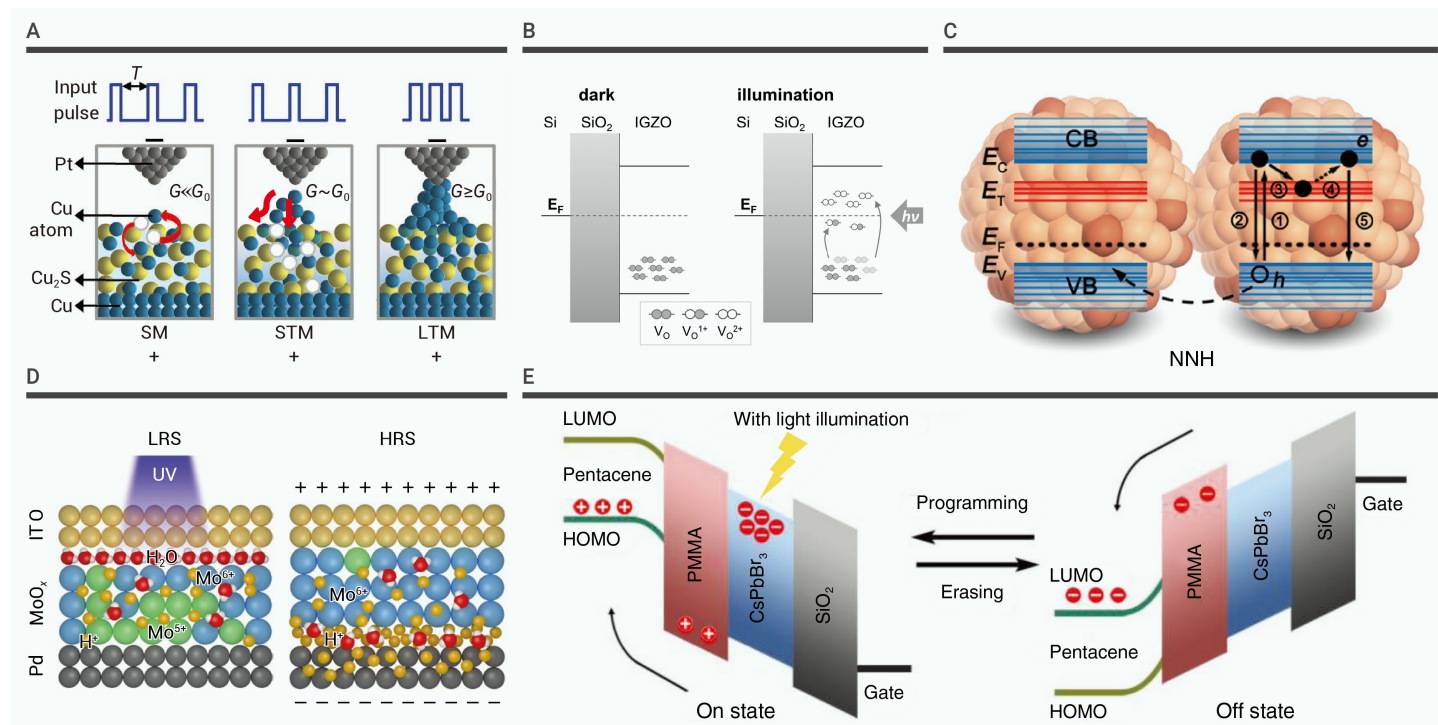
Figure 3. Energy band diagrams illustrating the mechanisms of various types of synaptic device (A) Ion mobility-based mechanisms. Reproduced with permission. 54 Copyright 2017, The Authors, distributed under CC BY 4.0. (B) Ionization and deionization of oxygen vacancies. Reproduced with permission. 56 Copyright 2017, WILEY - VCH. (C) Carrier trapping and release. Reproduced with permission. 57 Copyright 2018, Elsevier. (D) Photoinduced phase transitions. Reproduced with permission. 58 Copyright 2019, Springer Nature. (E) Electrically assisted photo stimulation. Reproduced with permission. 59 Copyright 2018, WILEY - VCH. Reproduced with permission. 60 Copyright 2018, WILEY - VCH.
