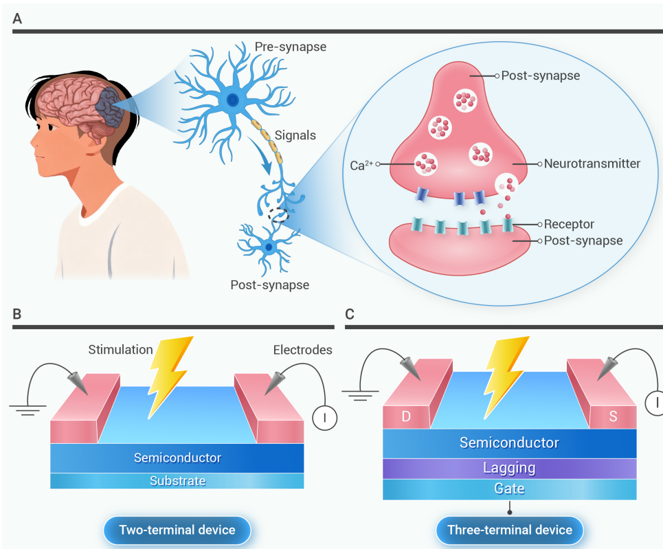
Figure 2. Schematic illustration of biological synapses and artificial synaptic devices (A) A schematic diagram illustrating the structure of a biological synapse. A schematic diagram illustrates the structure of the artificial synaptic devices with (B) two terminals, and (C) three terminals.
