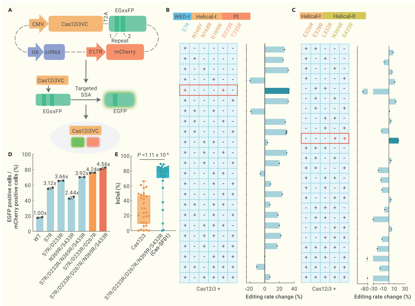
Figure 2. Cas-SF01 engineering via a 2-step combined strategy (A) Schematics of the EGxFP reporter system for screening for high-efficiency Cas12i3 variants carrying combinations of mutations (Cas12i3VC). A short sequence is inserted inside the EGFP to disrupt its fluorescence. Targeted cleavage in the inserted sequence restores EGFP fluorescence due to DNA repair through single-strand annealing (SSA) between 2 flanking repeats. The system also constitutively expresses an mCherry marker. Editing efficiency is assessed by determining the ratio of EGFP + cells over mCherry + cells. (B and C) The editing efficiencies of Cas12i3 with different mutation combinations for the PAM-interacting region (B) and target DNA strand-interacting region (C), as determined by the EGxFP reporter. The mutation combinations with the highest editing rate increase in the 2 regions are highlighted in red boxes. (D) Further combination of mutations identified from the screens results in variants with higher editing efficiency. The variant with highest editing efficiency contains 5 mutations (S7R/D233R/D267R/N369R/S433R) and was called Cas-SF01. (E) Comparison of indel activity of Cas12i3 and Cas-SF01 at the TTR locus in mammalian cells. Significant difference was determined by Student's t test.
