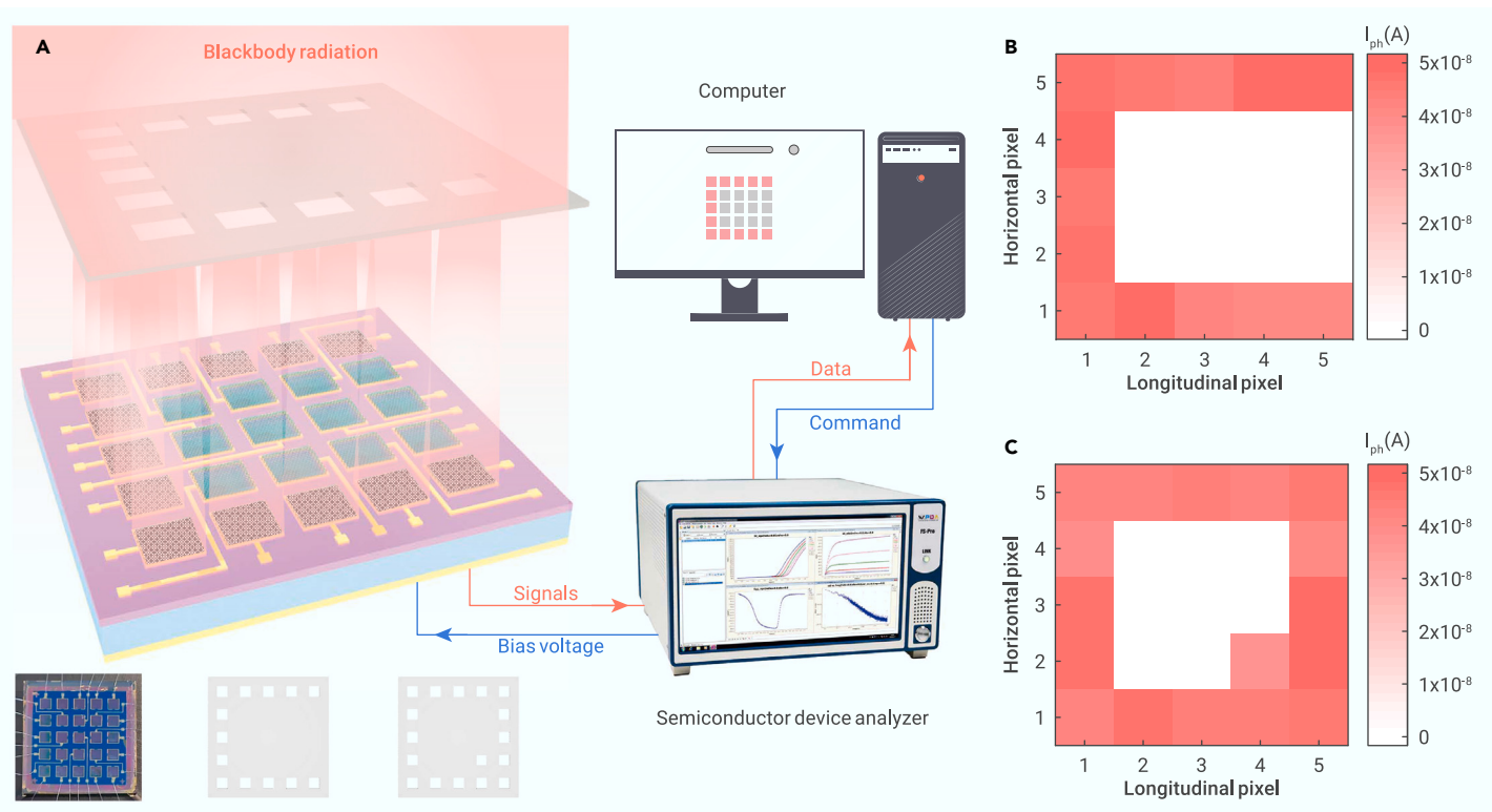
Figure 5. Photoresponse of the SPBD array (A) Top: schematic of the photoresponse measurement based on the device array. Bottom: photograph of the 5 × 5 device array and the schematics of the two custom masks representing “C” and “Q.” The photosensitive area of each pixel is 1 mm × 1 mm. The results of the letter pattern when using masks (B) “C” and (C) “Q” under 1,000 K blackbody radiation. The photoresponse of the SPBD array when using a light-emitting diode (LED) as a light source is shown in Figure S15, which exhibits similar results.
