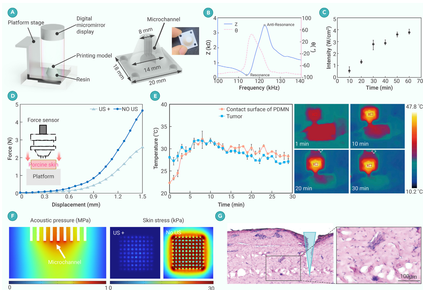
Figure 2. Characterization of the PDMN platform (A) Schematic diagram of the fabrication process of the MA patch by surface projection microstereolithography. (B) Impedance and phase angle spectra of PDMN. The impedance experiment is performed showing PDMN's excellent piezoelectricity. At the resonant frequency, the generator will be the most power efficient. Impedance and phase angle spectra of the PDMN probe after integration showing a center frequency of 114 kHz, an anti-resonance frequency of 122.5 kHz, a phase angle of 80°, and an electromechanical coupling factor k_t of 0.53. (C) Correlation between intensity and time. (D) Mechanical behavior of PDMN against compressive deformation. (E) Temperature changes of PDMN operated for 30 min measured by an infrared thermal camera. Time-temperature curves (left) and representative temperature profiles were captured by a thermal camera every 10 min (right). (F) Finite element method simulation of acoustic pressure and stress field under the skin coupled with PDMN. (G) Representative H&E staining images of porcine skin under PDMN treatments. Scale bar, 100 μm.
