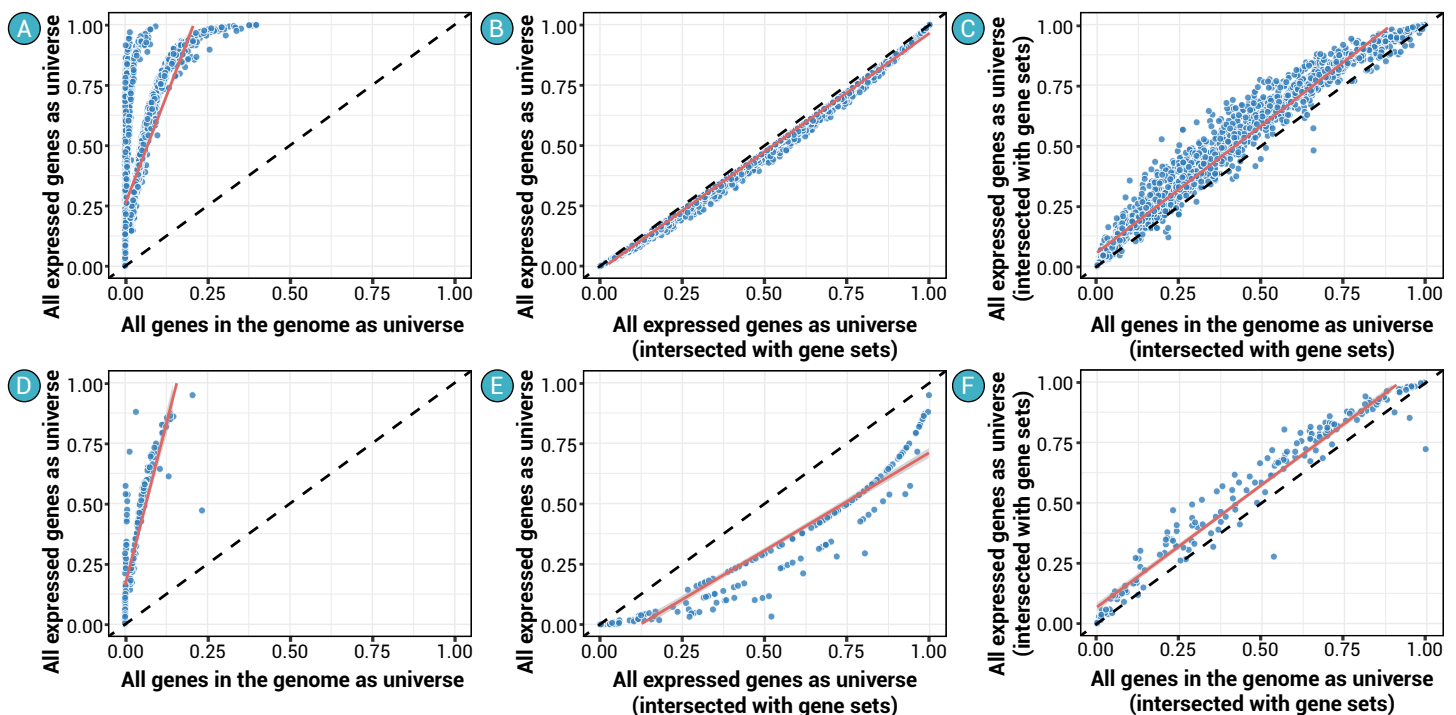
Figure 1. Comparison of enrichment p -values under different background universes and strategies (A, D) Using all expressed genes as the universe versus using all genomic genes as the universe. (B, E) Using all expressed genes as the universe versus using the intersection of expressed genes and the gene set as the universe. (C, F) Using the intersection of expressed genes and the gene set as the universe versus using the intersection of all genomic genes and the gene set as the universe. Panels A–C show results from Gene Ontology (biological process) enrichment analysis, whereas panels D–F show results from KEGG pathway analysis. Reproducible analysis scripts for Figure 1 are available at: https://github.com/YuLab-SMU/Background-bias-of-functional-enrichment-analysis .
